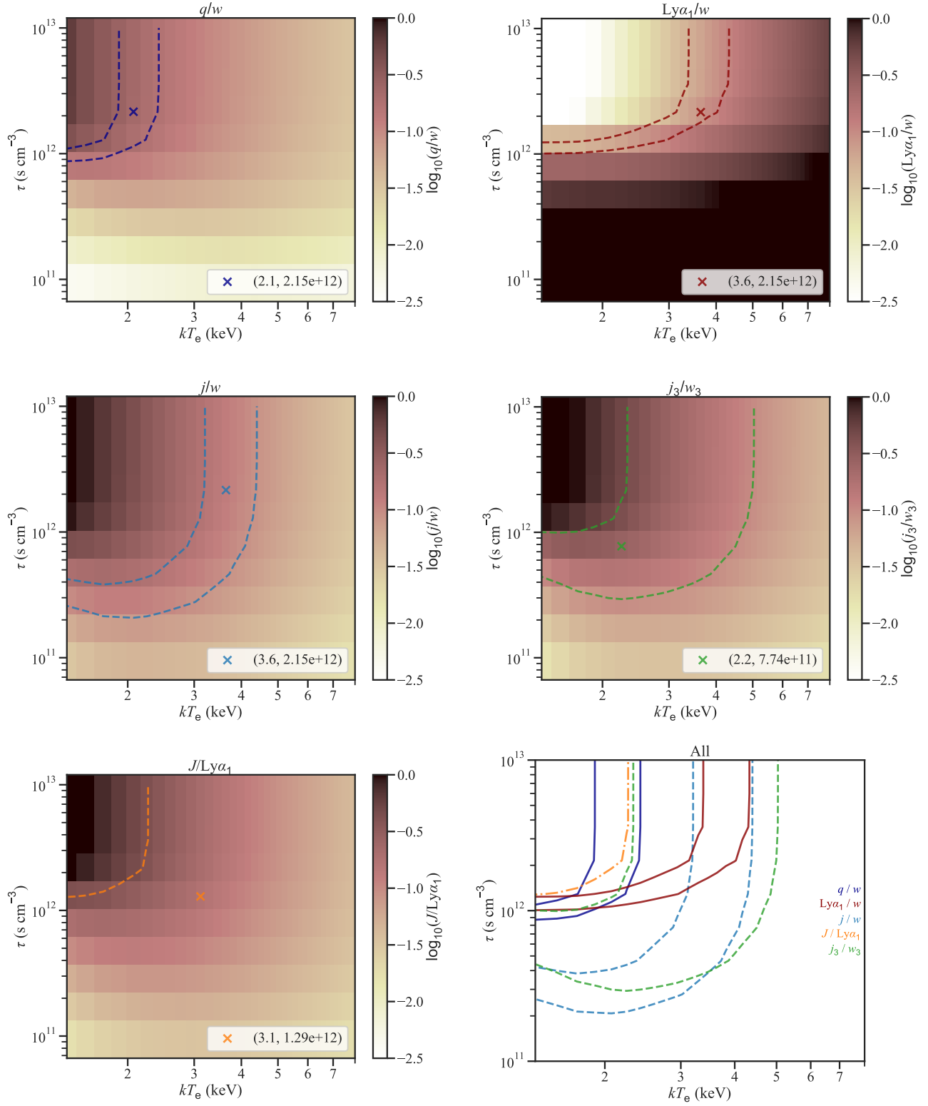
Fig. 11. Diagnostics for the recombining plasma. The format and symbols follow 9. The ionizing plasma model in AtomDB is retrieved via PyAtomDB (Foster & Heuer 2020) to calculate the five line ratios as functions of the relaxation parameter \tau and the electron temperature kT_e . The initial condition at \tau = 0 assumes that all Fe ions are fully ionized and the electrons have a temperature of kT_e . No space satisfies all the contours simultaneously. Alt text: a six-panel figure of heatmaps showing kT_e on the x-axis and \tau on the y-axis.
