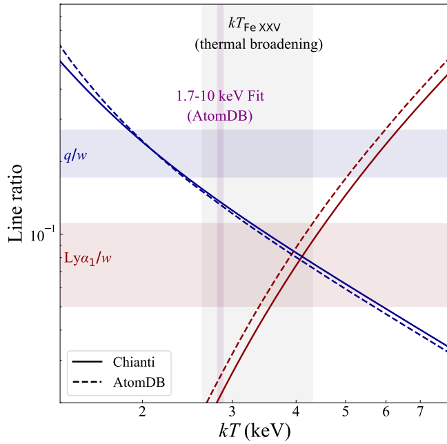
Fig. 6. Temperature diagnostics using line ratios sensitive to ion charge distribution. The line ratios of q/w (Li-like/He-like Fe) and \text{Ly}\alpha_1/w (H-like/He-like Fe) are shown in blue and red, respectively, for the observation (shaded areas) and calculation using Chianti (solid curves) and AtomDB (dashed curves). The best-fit kT from the broadband fitting using AtomDB (§ 3.2.1) and kT_{\text{FeXXV}} derived from the line broadening in the \text{He}\alpha complex are also presented. Alt text: A graph showing temperature on the x-axis and line ratio on the y-axis.
